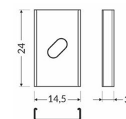
MOUNTING PLATE U INOX
