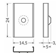
MOUNTING PLATE U CONE INOX
