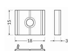
MOUNTING PLATE X
